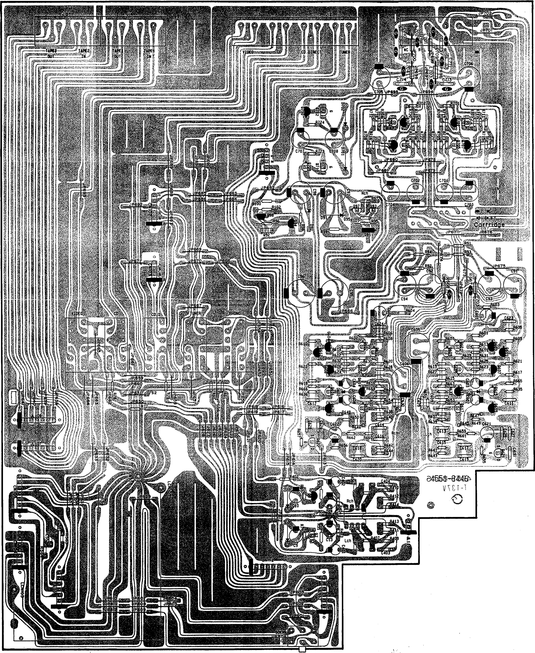
PCB-4 Pre Amp. P. C. Board
