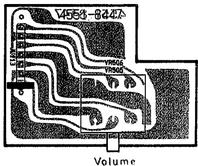
PCB-5 Volume P. C. Board
