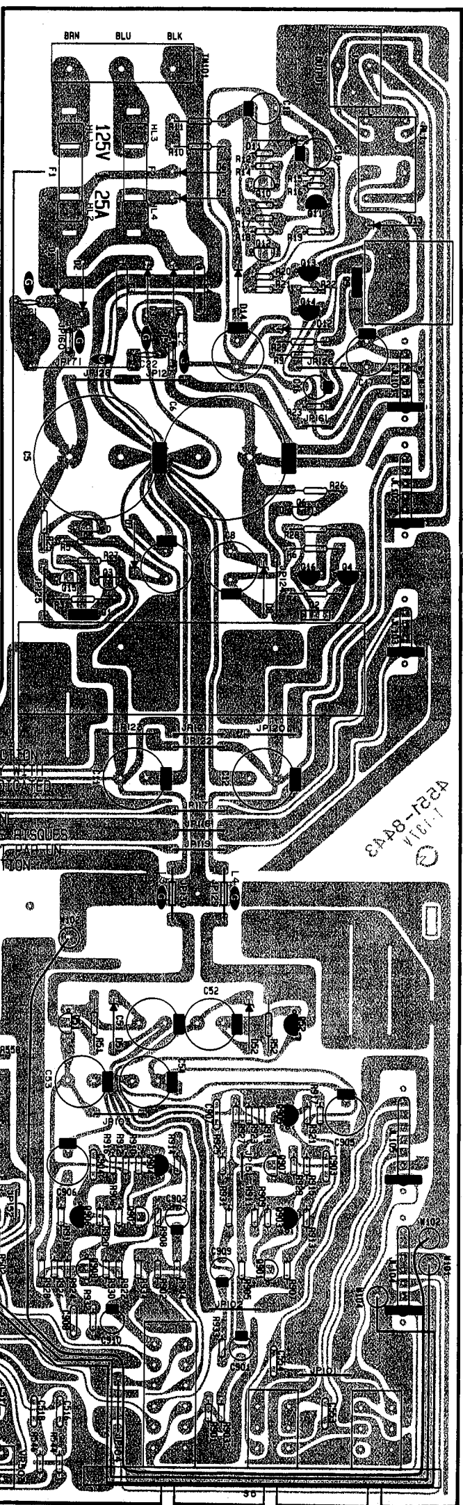
PCB-1 Power Supply P. C. Board
